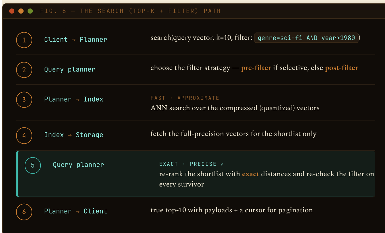
FIG. 6 — The two-phase pattern: cheap approximate narrowing, then exact precision on the shortlist.
