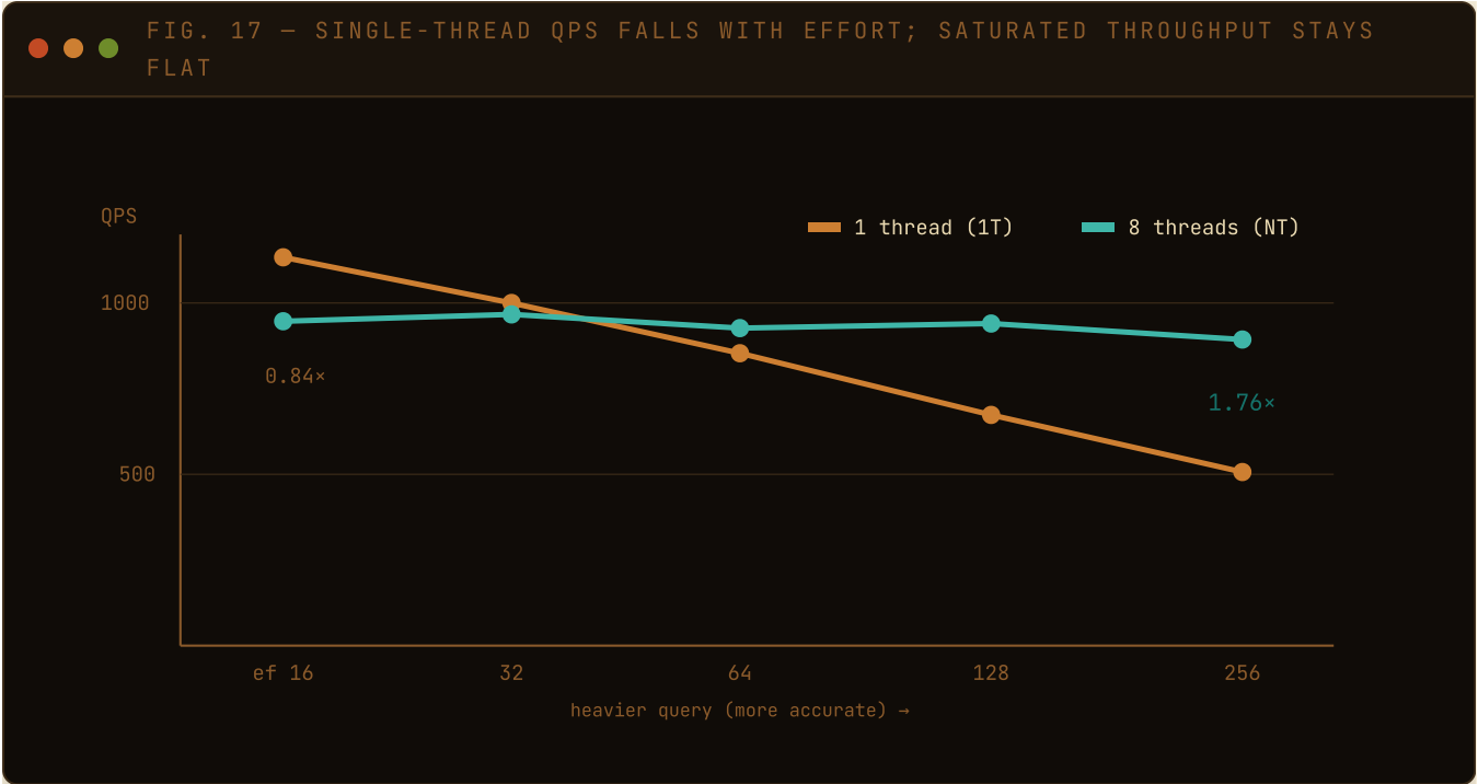
FIG. 17 – As queries get heavier, the single client thread (bronze) falls from 1131 to 506 QPS while the 8-thread server throughput (verdigris) holds near 900 – so the lines cross and saturated throughput pulls ahead, 1.76× at ef=256.
