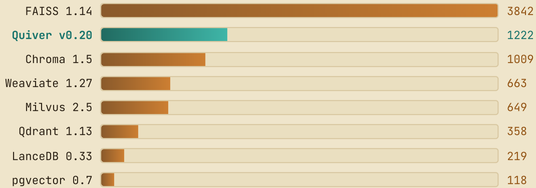
FIG. 16 — Single-thread QPS at recall@10 \geq 0.95 (v0.20.0). Quiver is second only to FAISS , with the field's second-best tail latency (1.0 ms).
