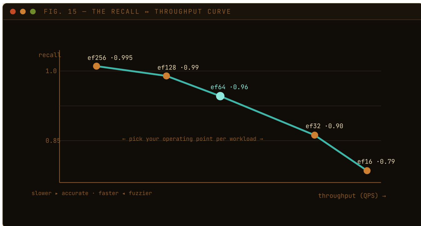
FIG. 15 – RAG pipeline that re-ranks anyway? Run at ef=64. Legal discovery where a miss is unacceptable? ef=256.
