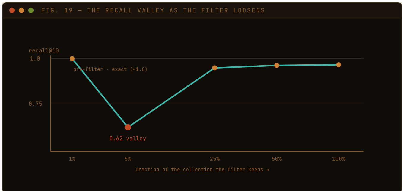
FIG. 19 — Always correct, never wrong: the filter is re-checked on every survivor (§4.5), so the “valley” is a recall dip the planner trades for speed, not an incorrect answer. Very selective filters pay in scan latency instead.
