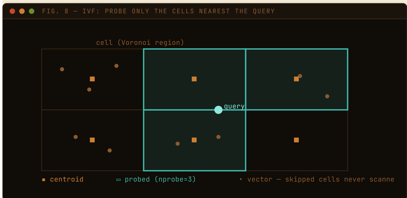
FIG. 8 — nprobe (how many cells to check) is IVF’s recall ↔ speed dial.
