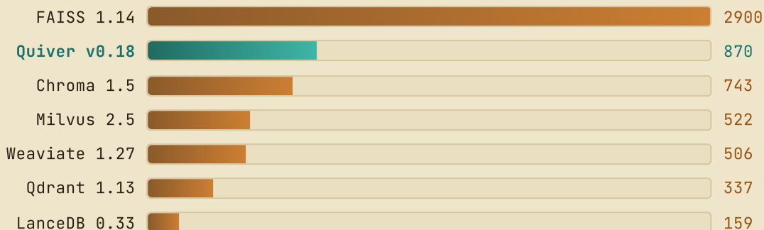
FIG. 14 — Single-thread QPS at recall@10 ≥ 0.95. Quiver is second only to FAISS , with the field’s second-best tail latency (1.5 ms).
