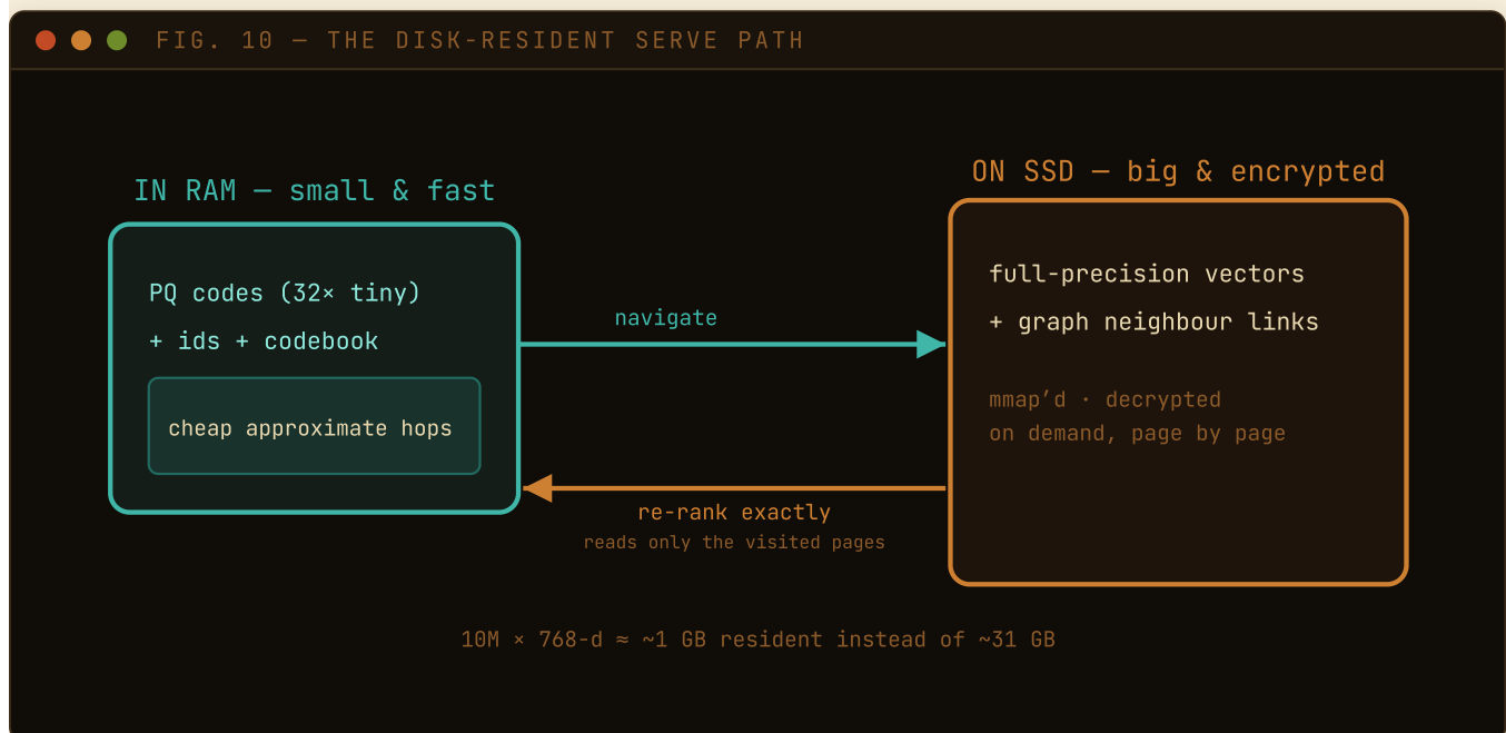
FIG. 10 — Only tiny PQ codes stay in RAM; full vectors and the graph live encrypted on SSD, touched only when visited.
