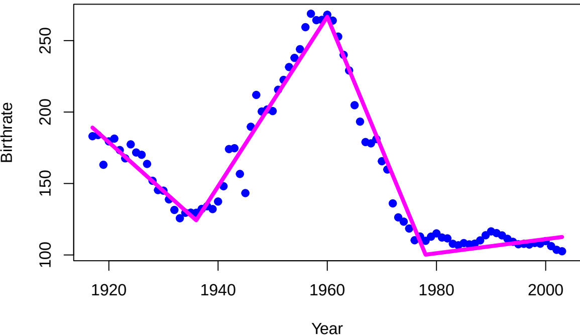
Linear spline with the bs() function
