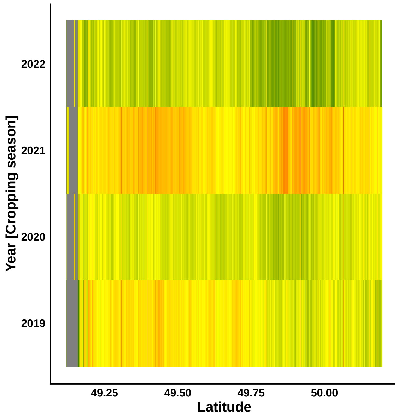
Lat Hovmöller Plot for Lightning , canola , 2022
