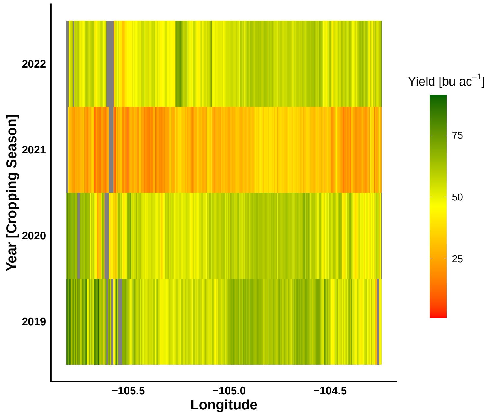
Longitudinal Hovmöller Plot for wheat_others
