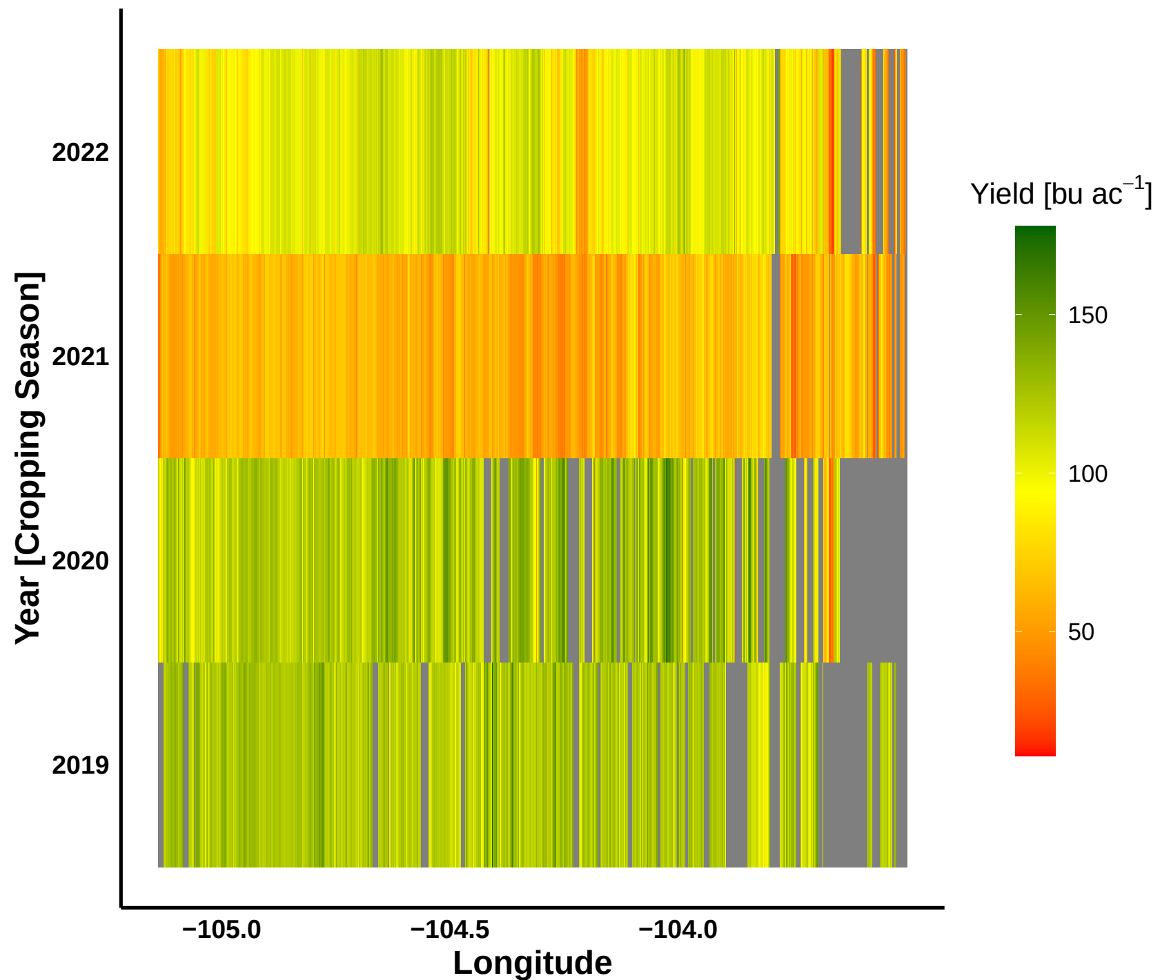
Lat Hovmöller Plot for Lenore Ponass , wheat_others , 2021 Longitudinal Hovmöller Plot for wheat_others
