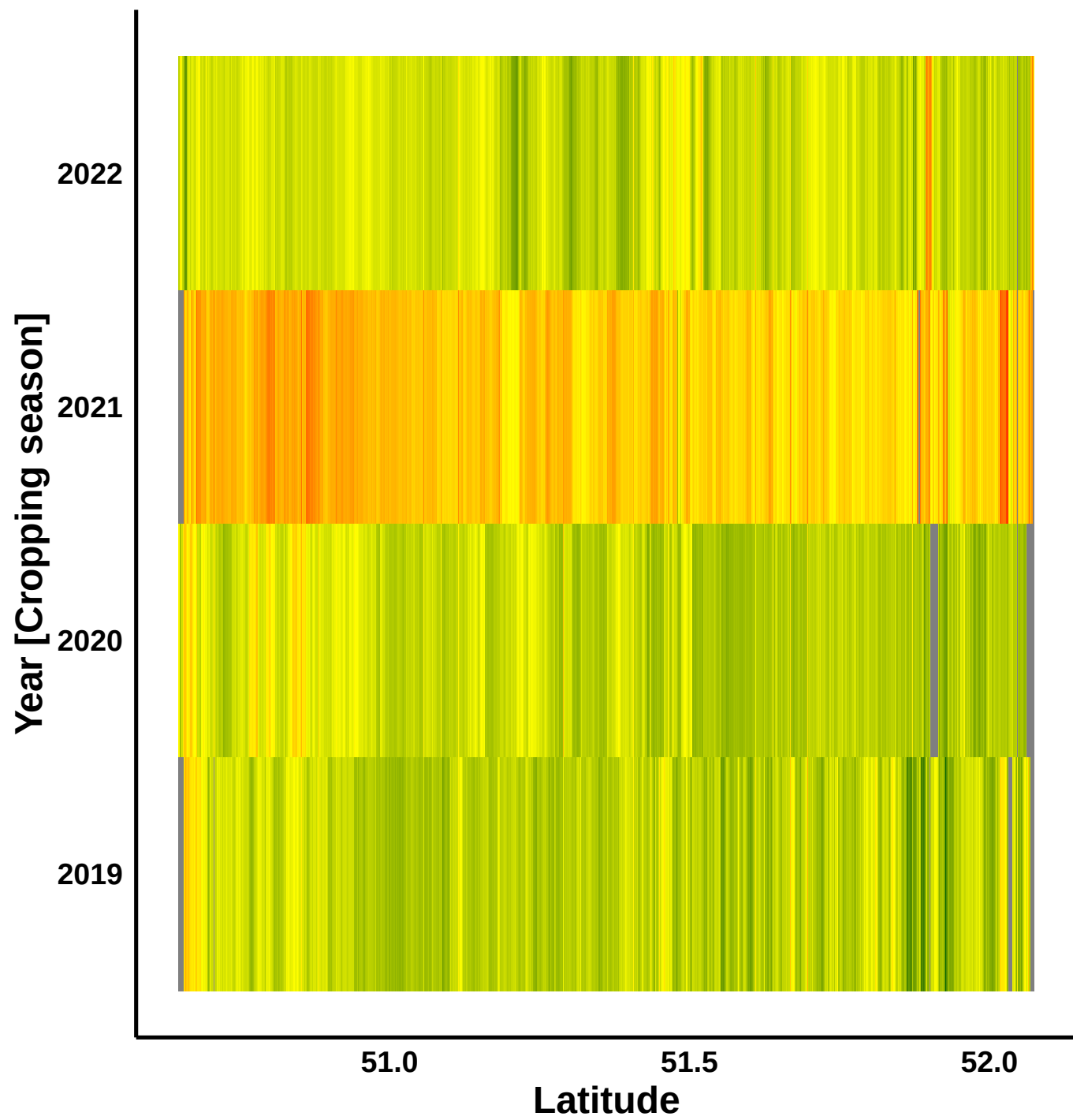
Lat Hovmöller Plot for Quill South , wheat_others , 2022
