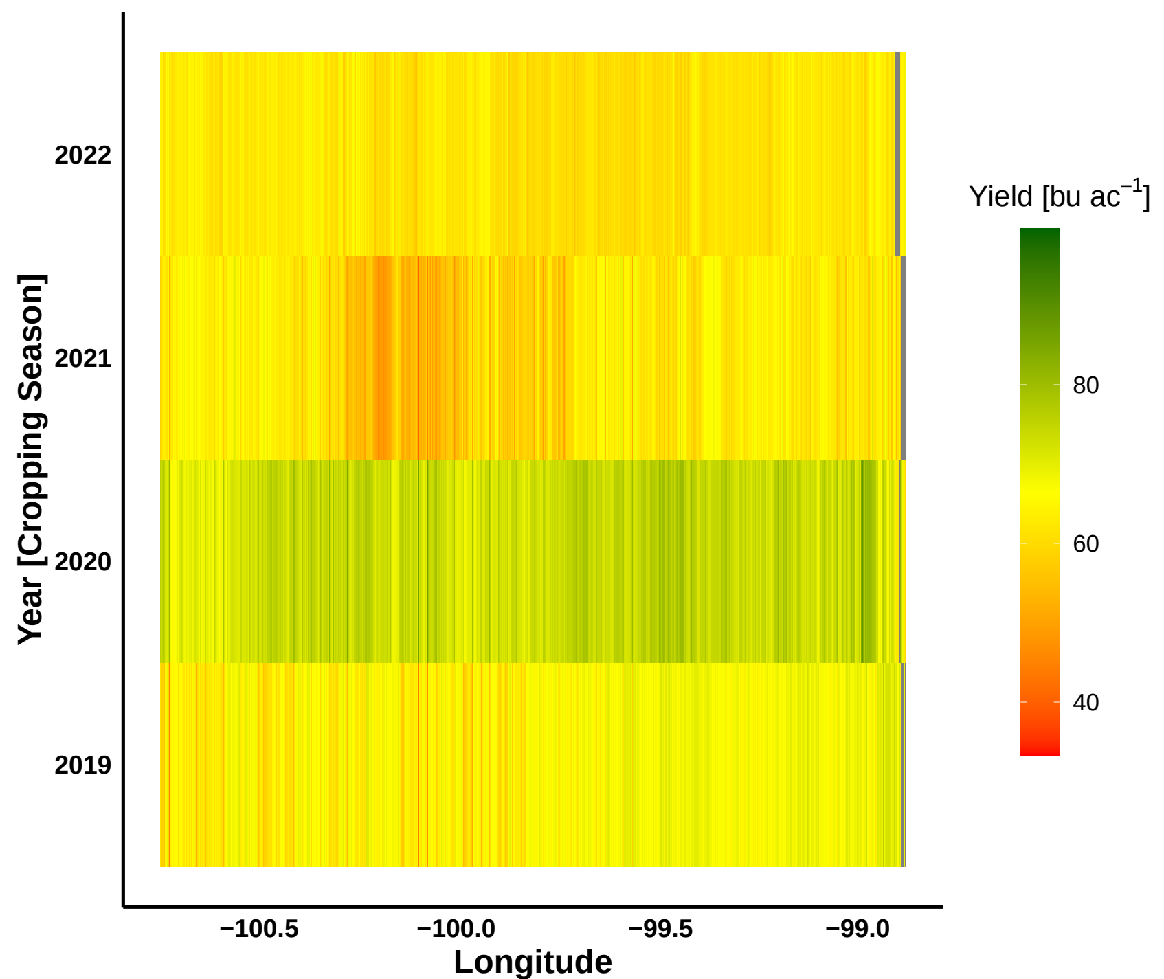
Lat Hovmöller Plot for Turtle Mountain , wheat_others , 2022 Longitudinal Hovmöller Plot for wheat_others
