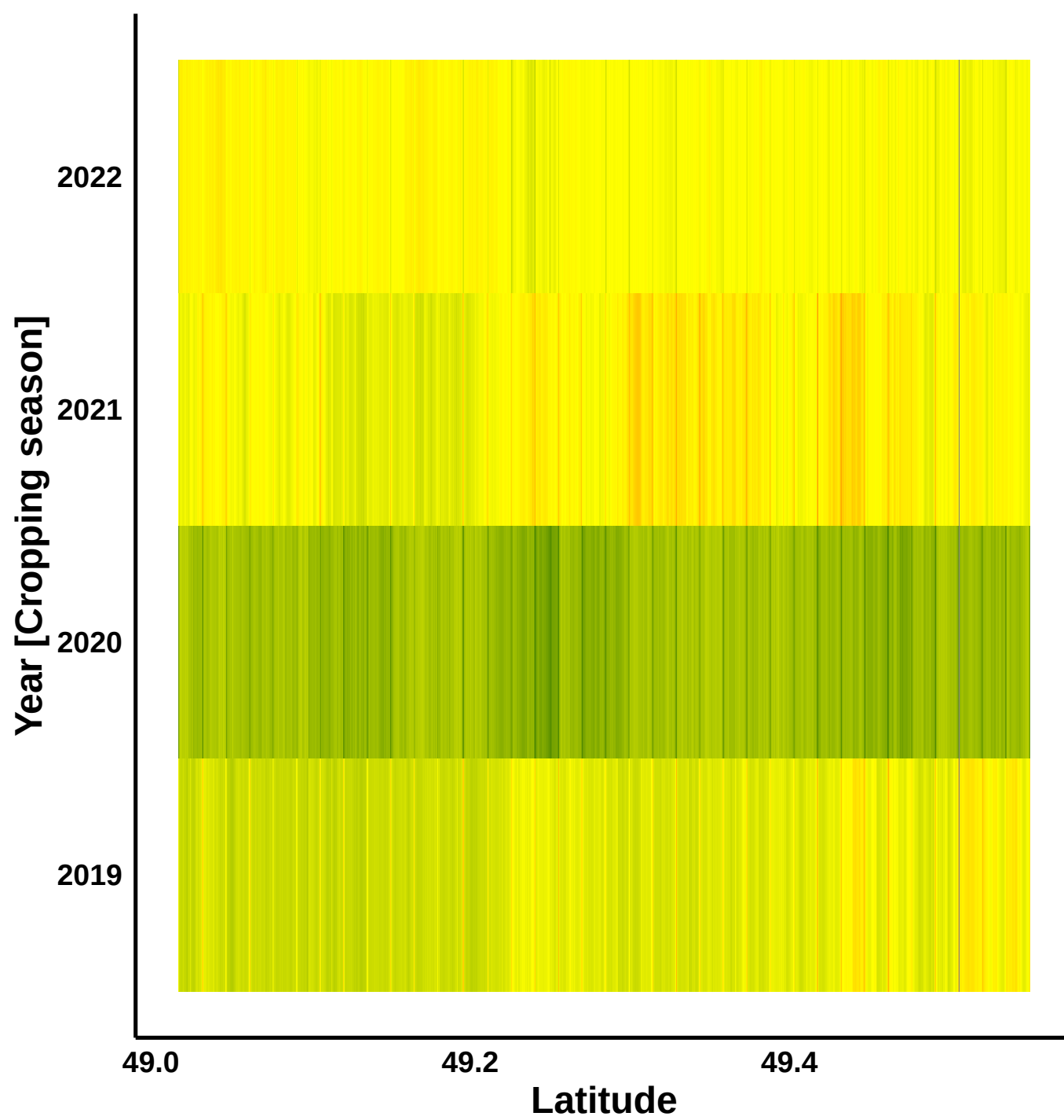
Lat Hovmöller Plot for Turtle Mountain , wheat_others , 2022 Longitudinal Hovmöller Plot for wheat_others
