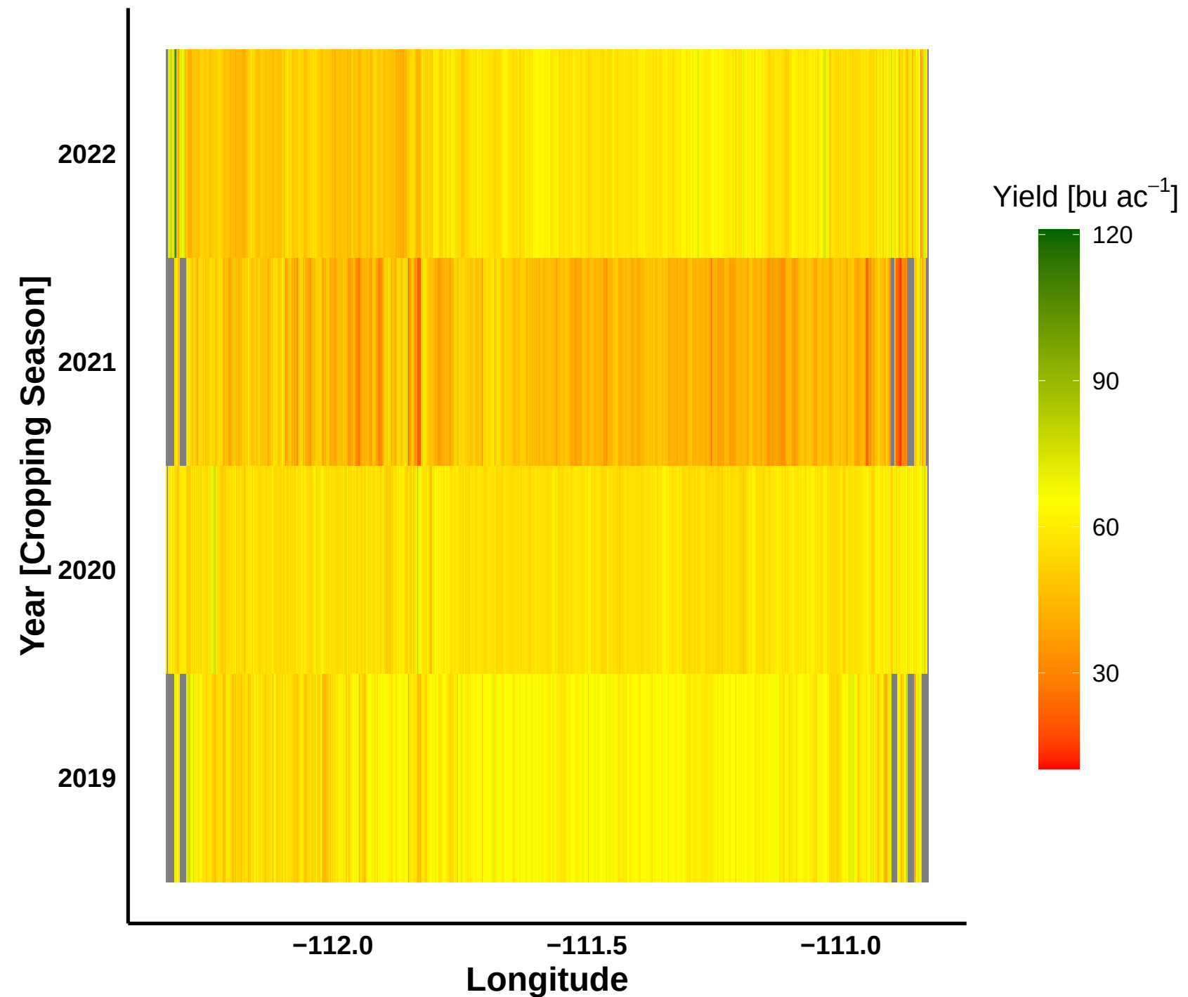
at Hovmöller Plot for Vermillion Viking , wheat_others , 2022 Longitudinal Hovmöller Plot for wheat_others
