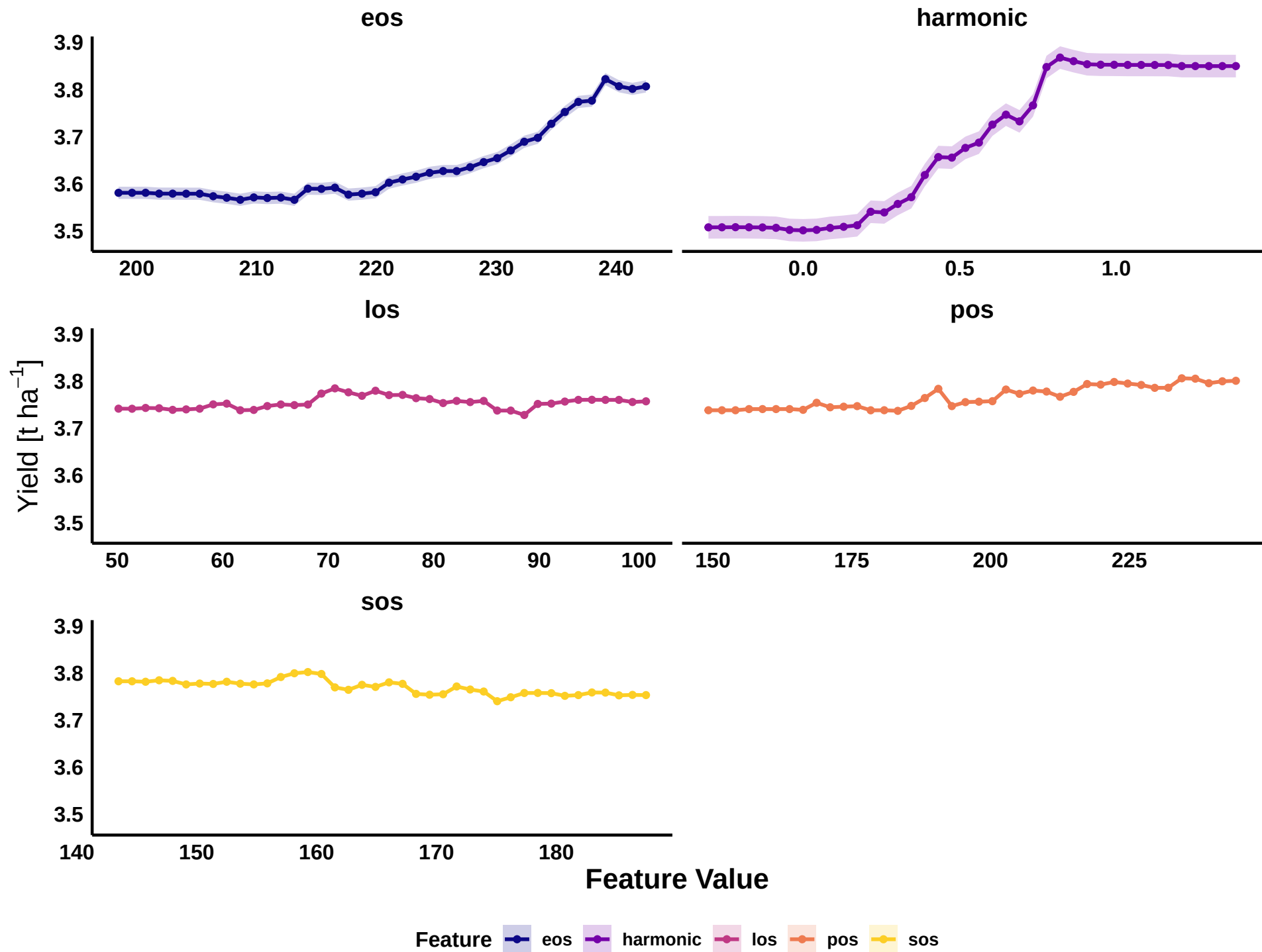
Partial Dependence Plots with \pm SE for wheat_others
