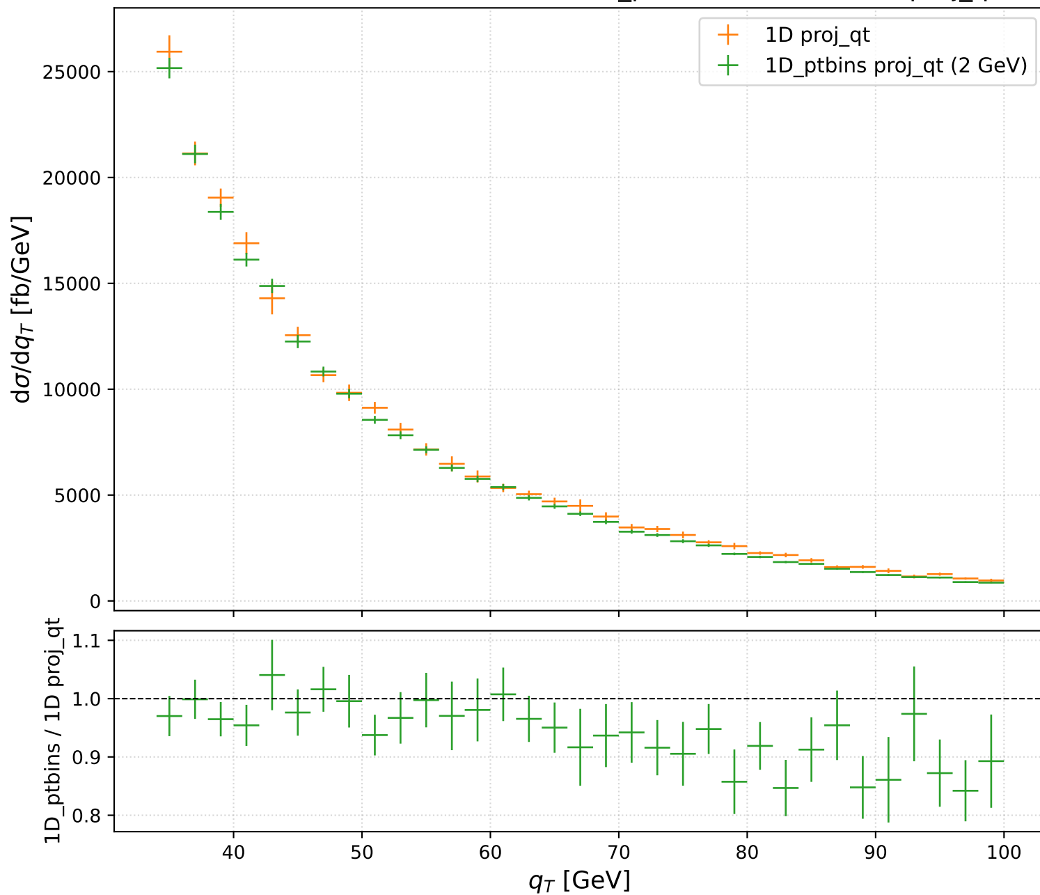
W^+ — N3LL, scala nominale — 1D\_{ptbins} (2 GeV) vs 1D proj\_qt
