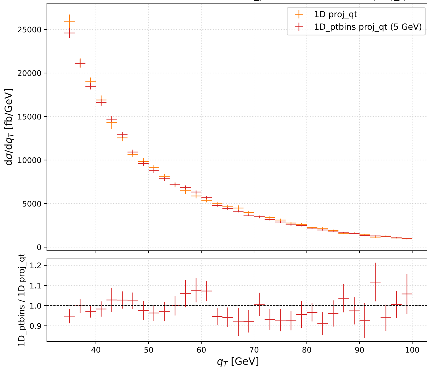
W^+ — N3LL, scala nominale — 1D\_ptbins (5 GeV) vs 1D proj_qt
