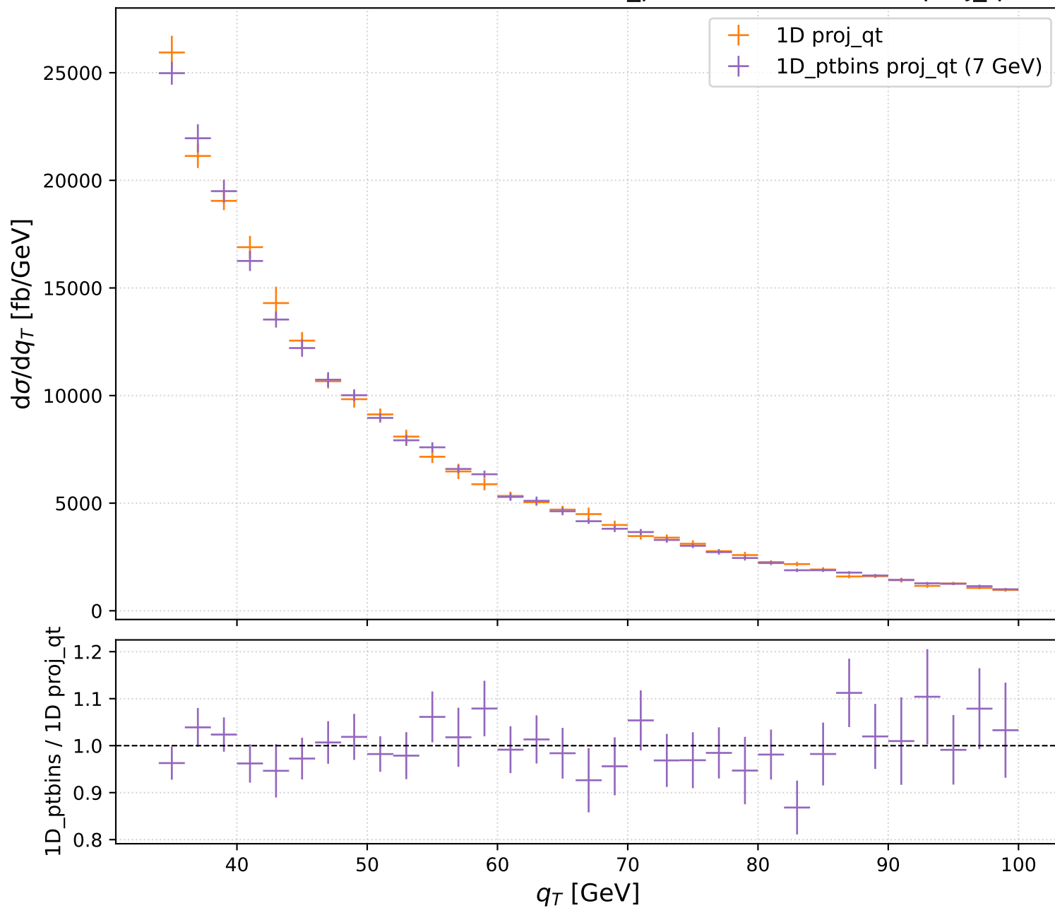
W^+ — N3LL, scala nominale — 1D\_{ptbins} (7 GeV) vs 1D proj\_qt
