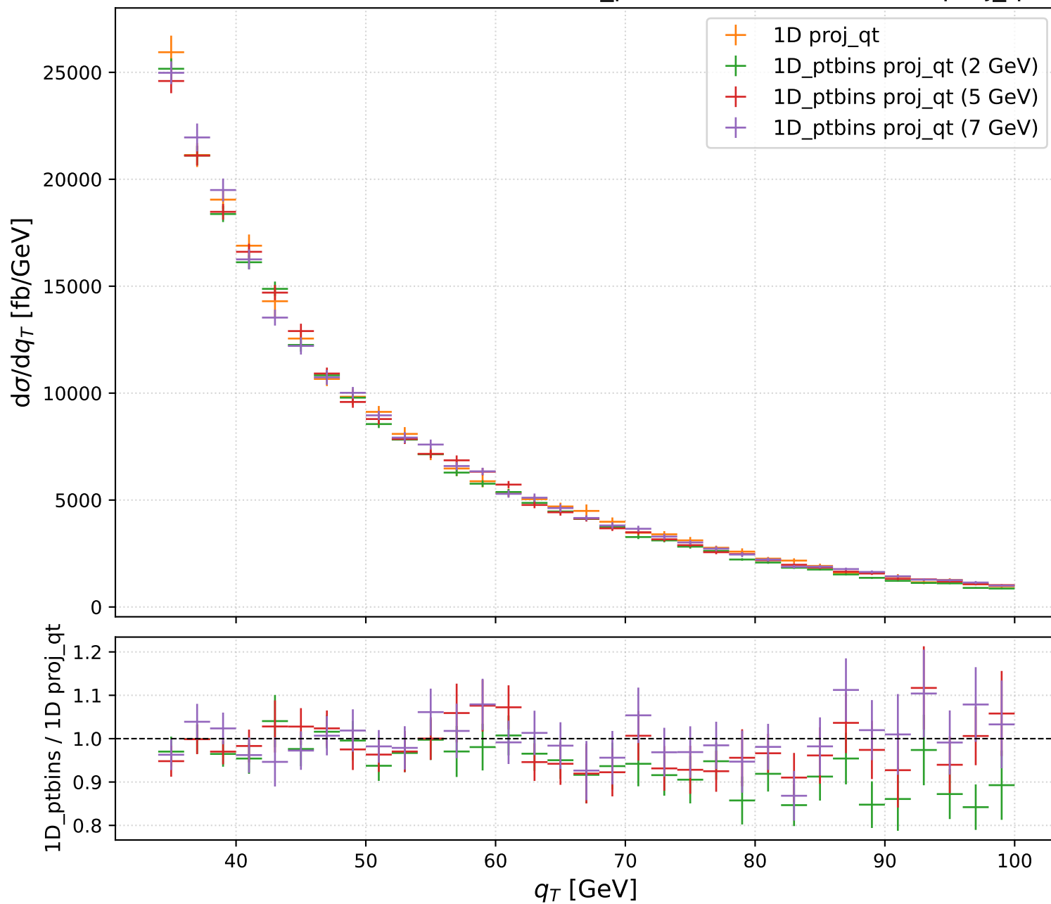
W^+ — N3LL, scala nominale — 1D_ptbins (2/5/7 GeV) vs 1D proj_qt
