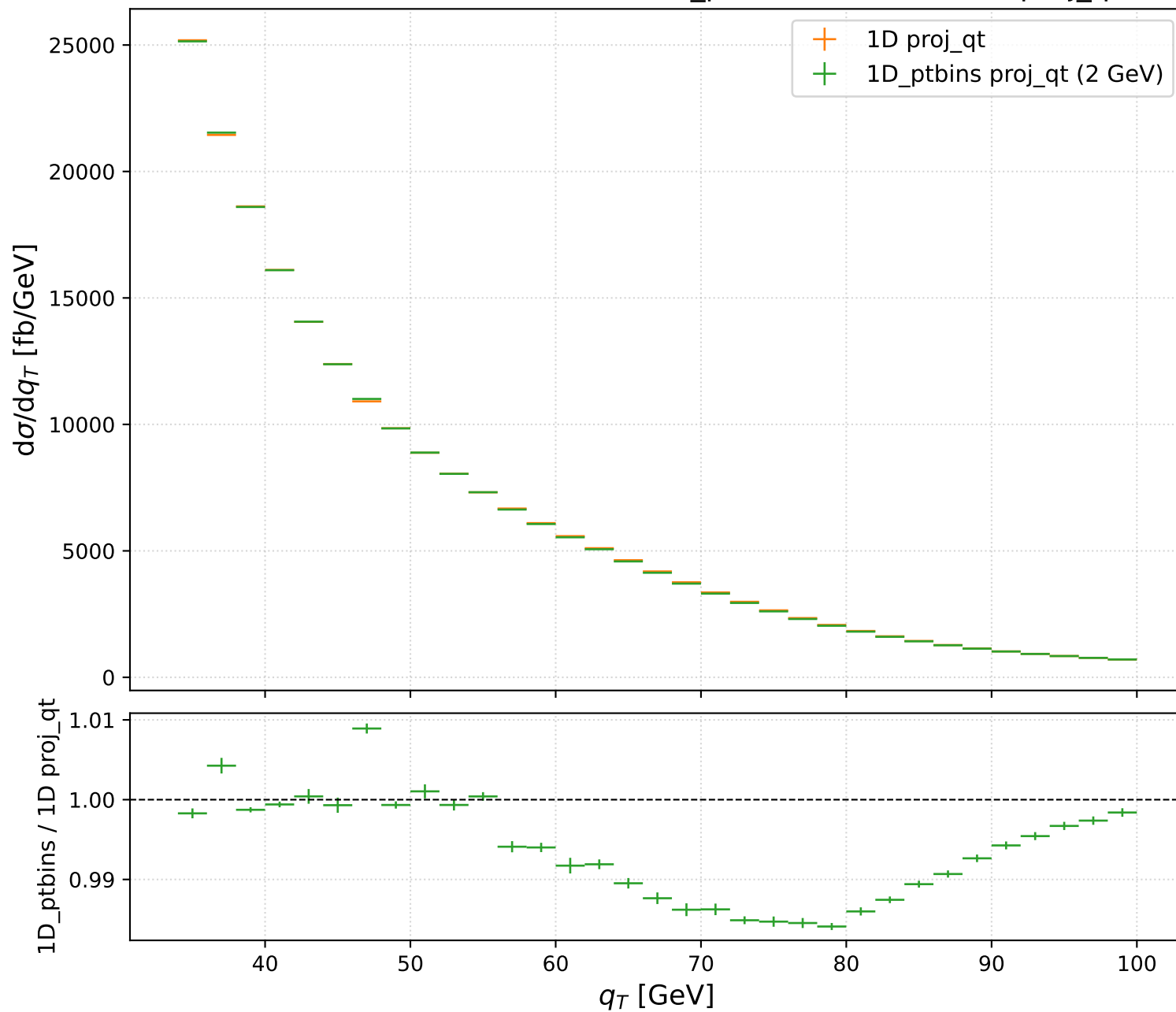
W^+ — NLL, scala nominale — 1D\_\_ptbins (2 GeV) vs 1D proj\_qt
