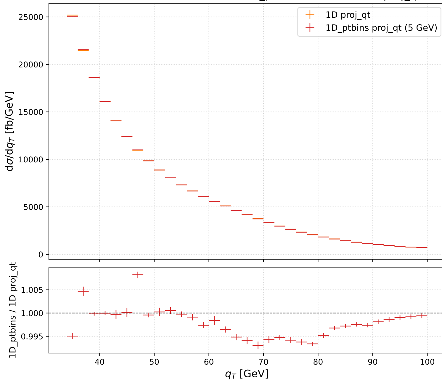
W^+ — NLL, scala nominale — 1D\_\_ptbins (5 GeV) vs 1D proj\_qt
