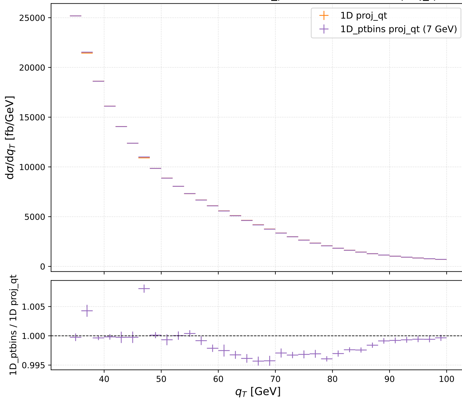
W^+ — NLL, scala nominale — 1D\_ptbins (7 GeV) vs 1D proj_qt
