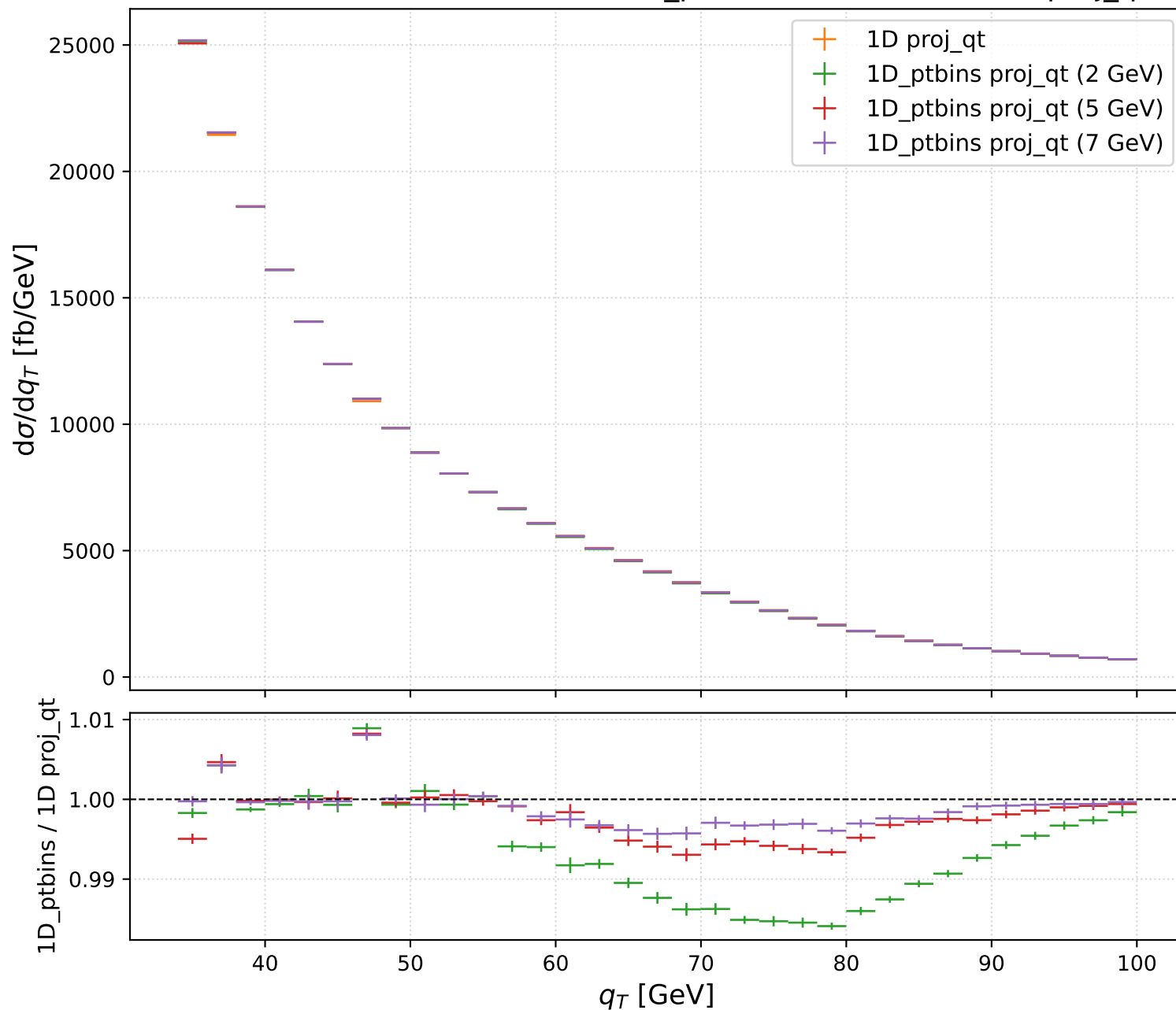
W^+ — NLL, scala nominale — 1D\_\_ptbins (2/5/7 GeV) vs 1D proj\_qt
