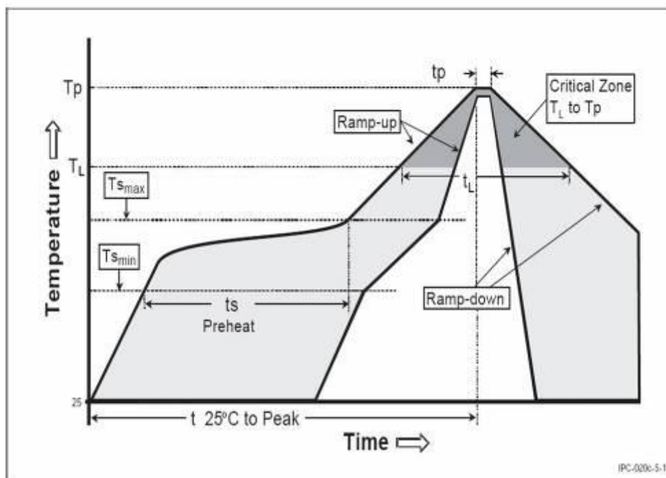
Figure 30: Soldering profile
