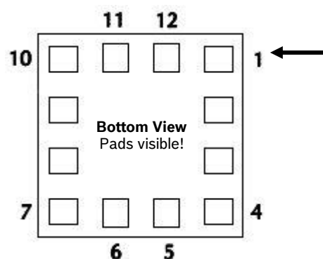
Figure 23: Pin-out bottom view
