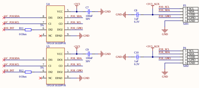
Senspr Board S201 &amp; 202 with passive filters
