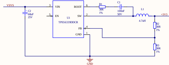
3V3 1A Regulator
