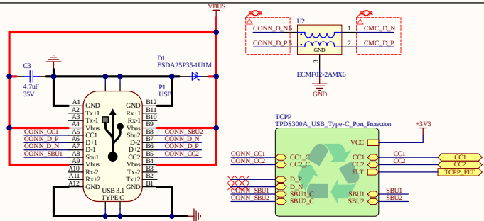
USB - C Section
