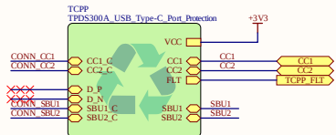
USB - C Section
