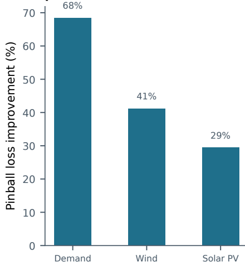
(b) Skill against climatology-persistence reference
