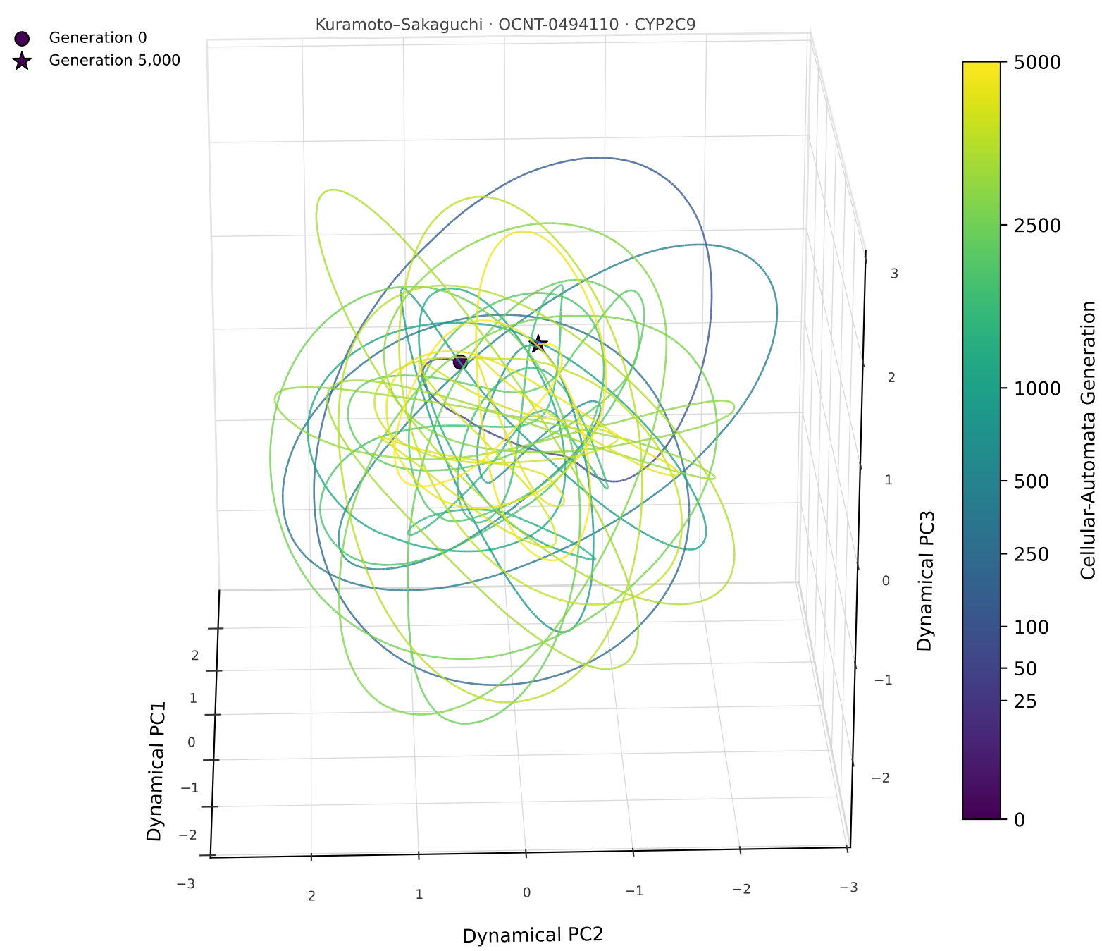
B | Trajectory 7: Strange Attractor
