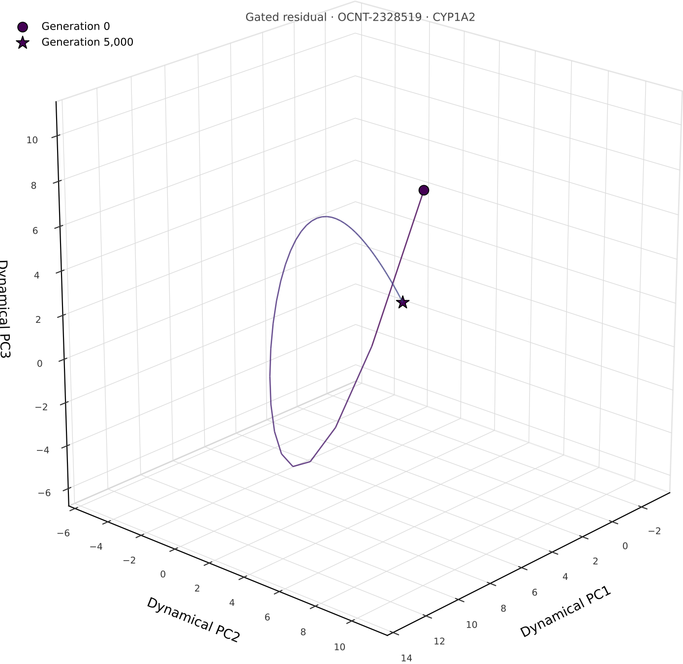
A | Trajectory 1: Point Attractor
