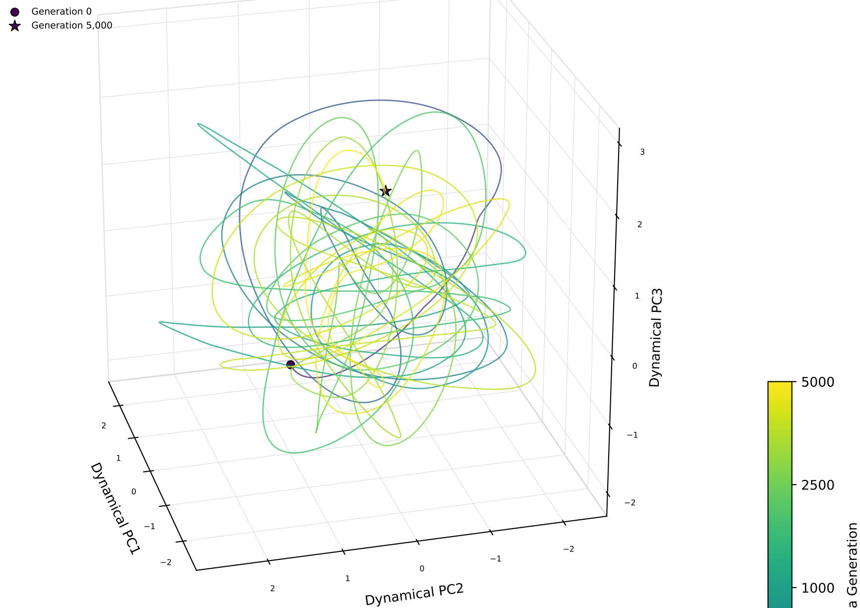
D | Period-2 Oscillator Candidate
