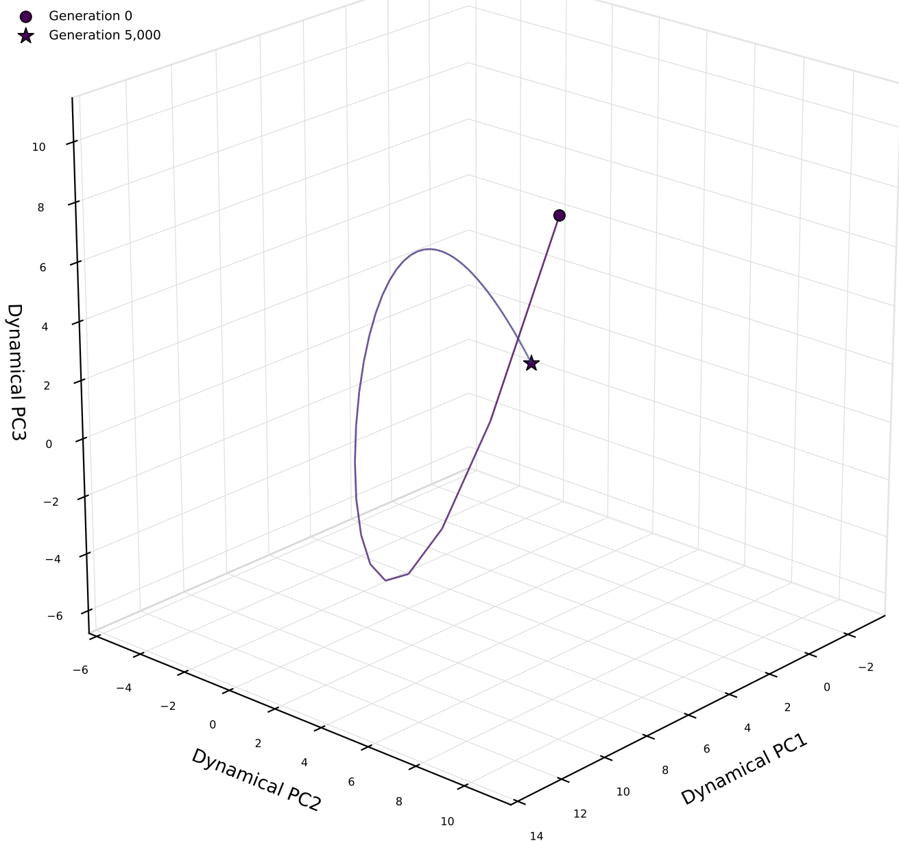
C | Persistent or Complex Candidate
