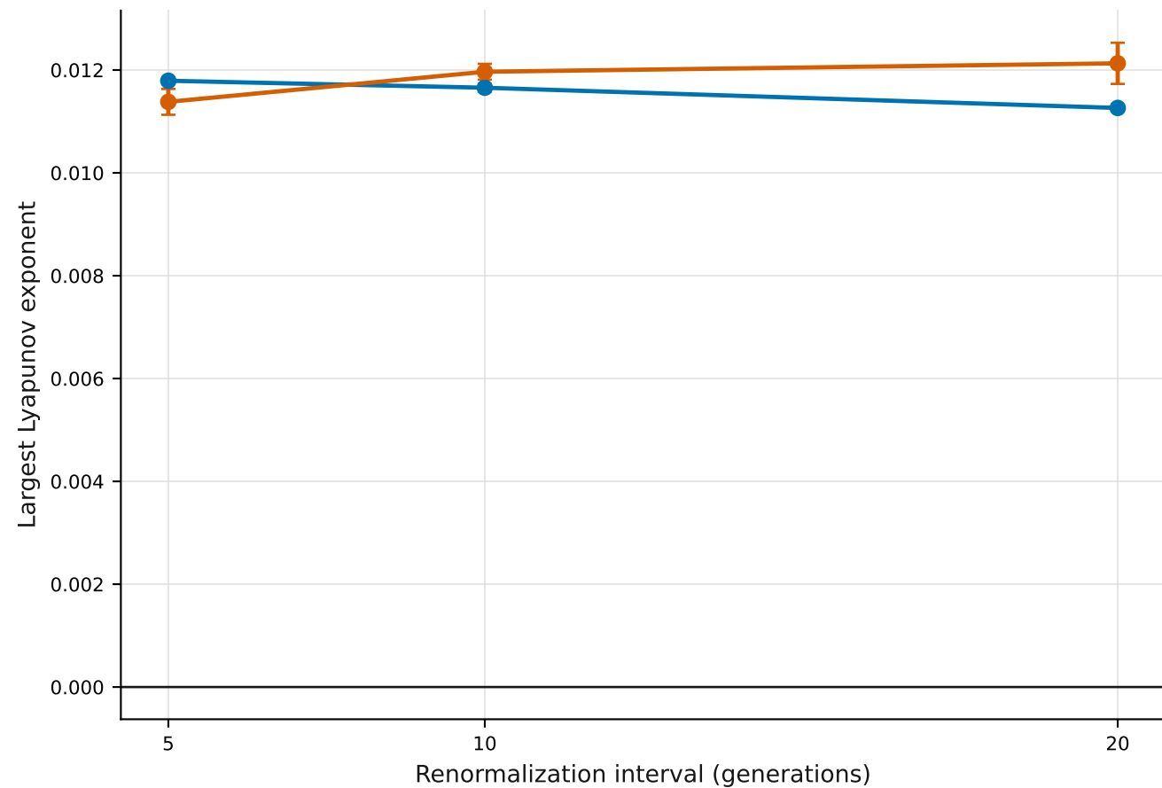
C | Exponent stability across calculation intervals
