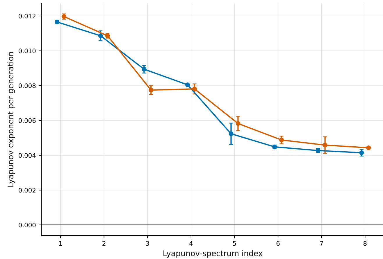
B | Eight positive Lyapunov exponents
