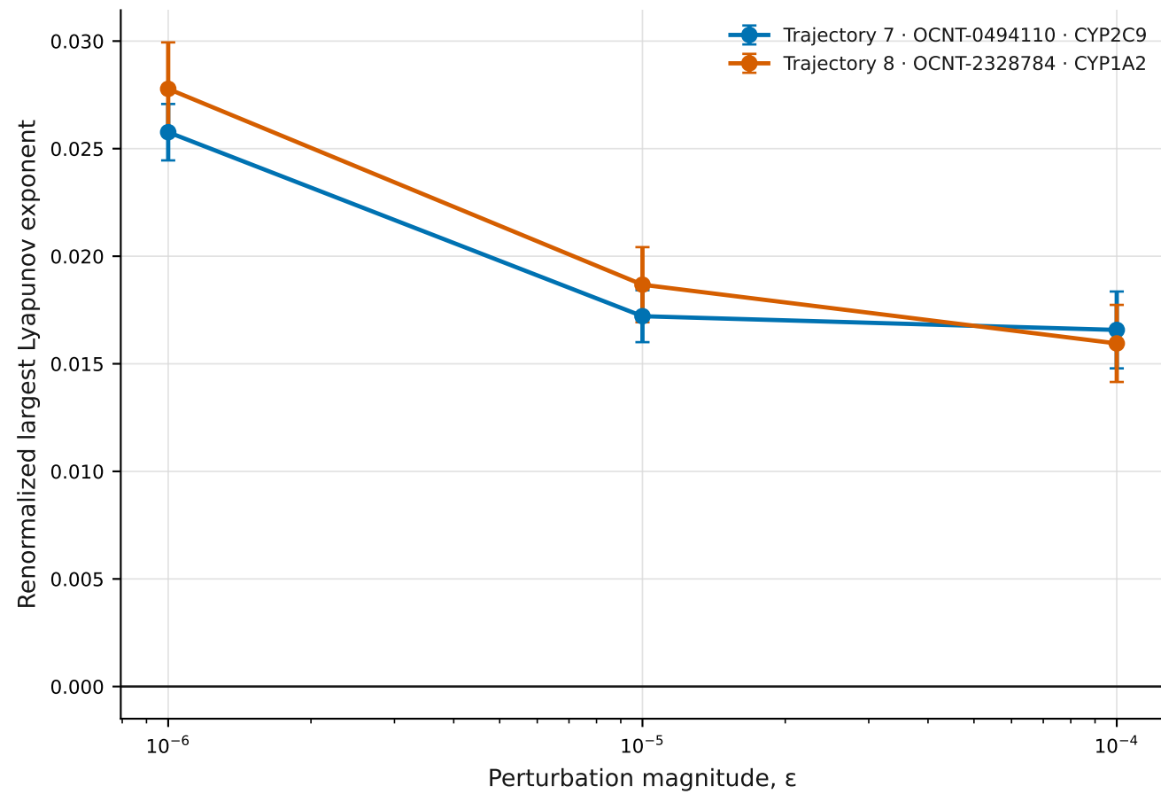
A | Continually regenerated divergence
