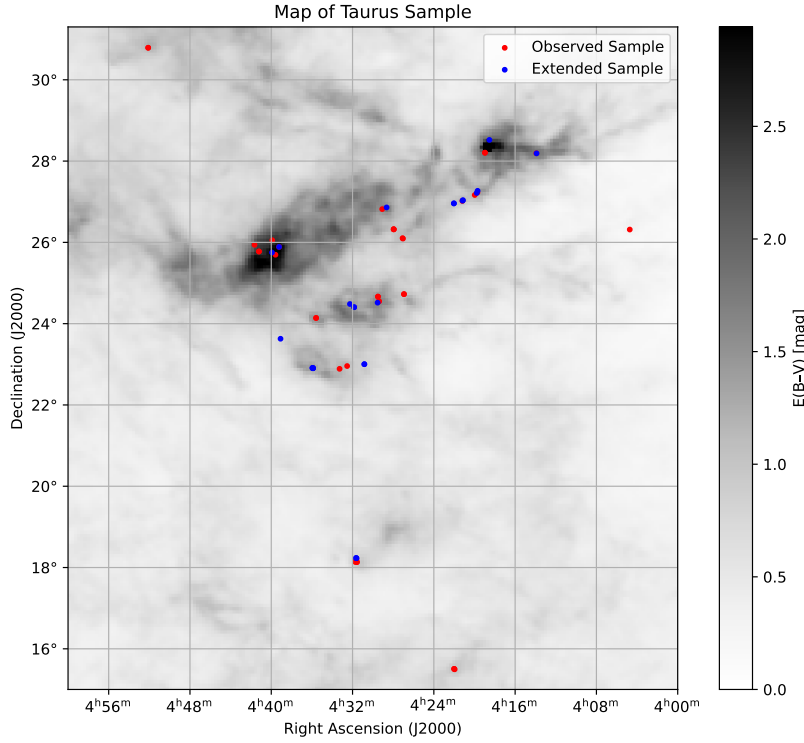
Figure 1. Map of the Taurus Molecular Cloud showing the locations of the sources overlaid on a background extinction map from D. J. Schlegel et al. (1998). Sources from the original sample are shown in red, and additional sources included in the Taurus+ sample are shown in blue.
