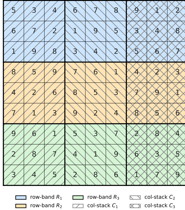
Sudoku base 1 with row-band and column-stack overlays
