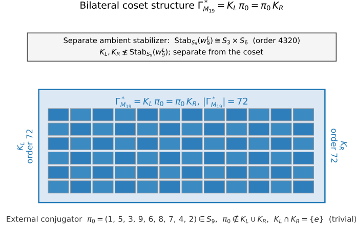
Figure 5: Schematic of the single-coset structure of \Gamma_{M_{19}}^* . The left axis is the |K_L| = 72 direction; \Gamma_{M_{19}}^* = K_L \cdot \pi_0 is itself a single left K_L -coset of cardinality 72. The structural permutation \pi_0 \in \Gamma_{M_{19}}^* also satisfies \Gamma_{M_{19}}^* = \pi_0 \cdot K_R ; the conjugation K_L = \pi_0 K_R \pi_0^{-1} identifies the two affine sides.
