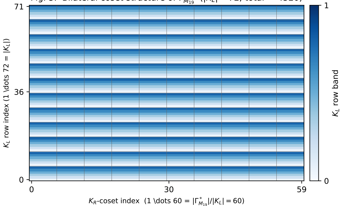
Fig. 5. Bilateral coset structure of \Gamma_{M_{19}}^* ( |K_L| = 72 , total = 4320)
