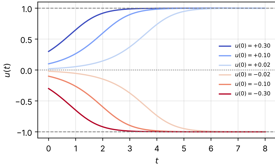
gradient flow \dot{u} = u - u^3 : same equation, opposite outcome depending on sign of perturbation
