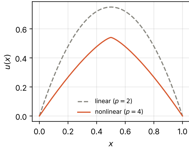
linear vs. p -Laplacian, same f = 6
