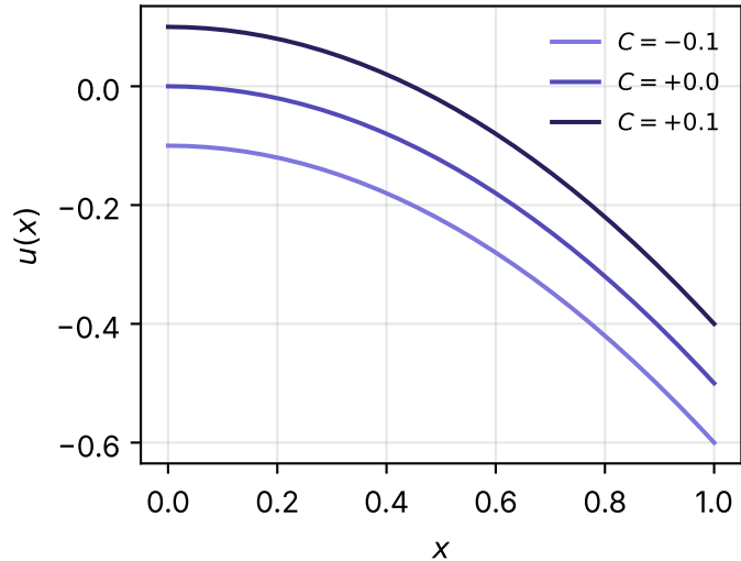
pure Neumann: unique up to a constant
