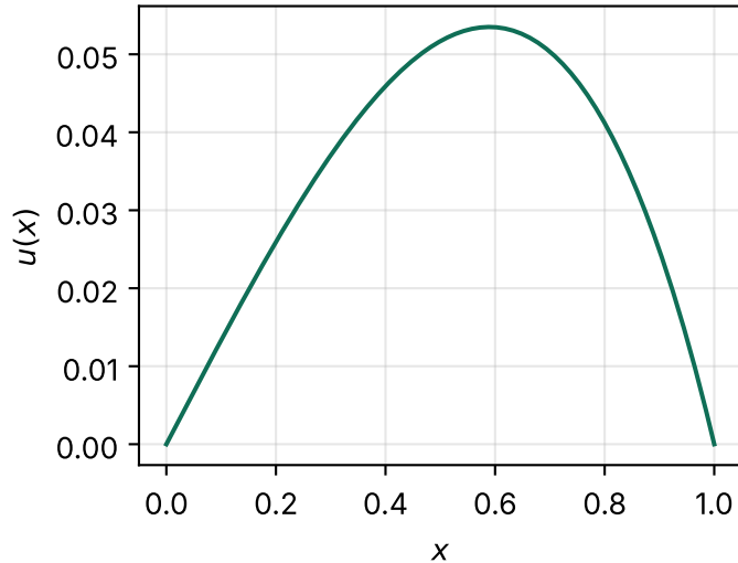
-u'' + 2u = x u(0) = u(1) = 0
