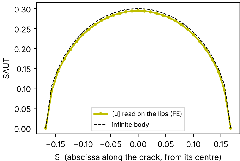
FIG 3 opening [u1] on the crack
