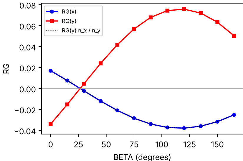
FIG 9 the two columns of R are proportional
