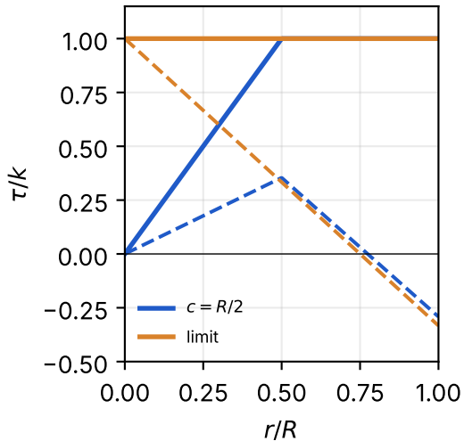
(b) torsion of a shaft
