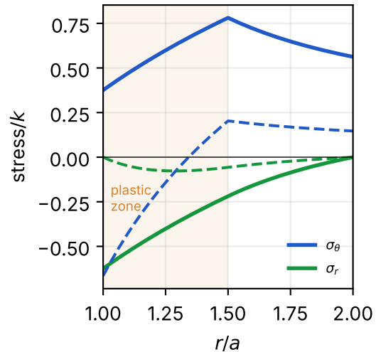
(a) thick cylinder, b = 2a , c = 1.5a
