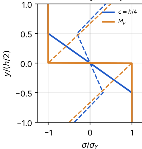
(c) bending, \varepsilon = -\kappa y
