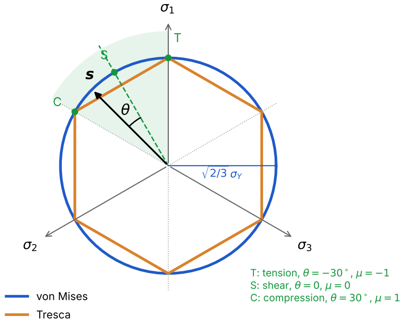
(b) deviatoric ( \pi ) plane and Lode angle
