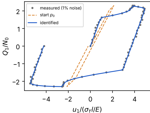
(a) response of the truss
