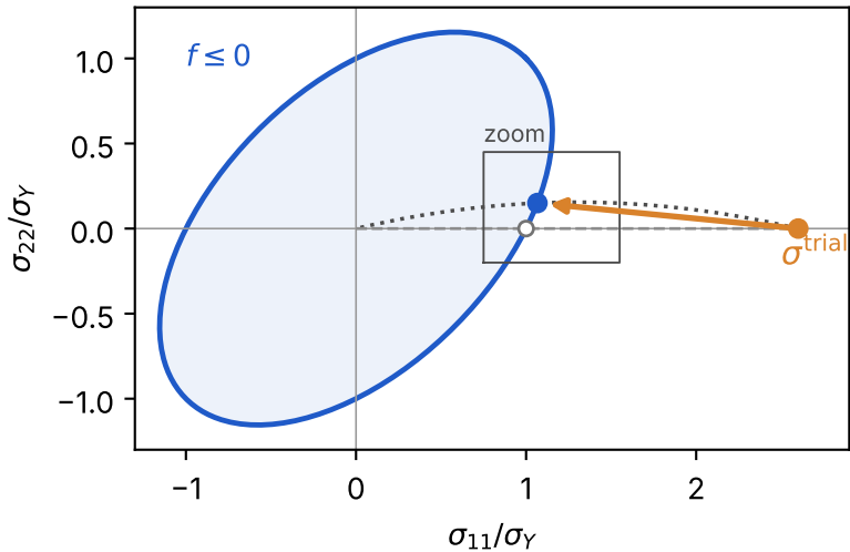
(a) principal plane stresses
