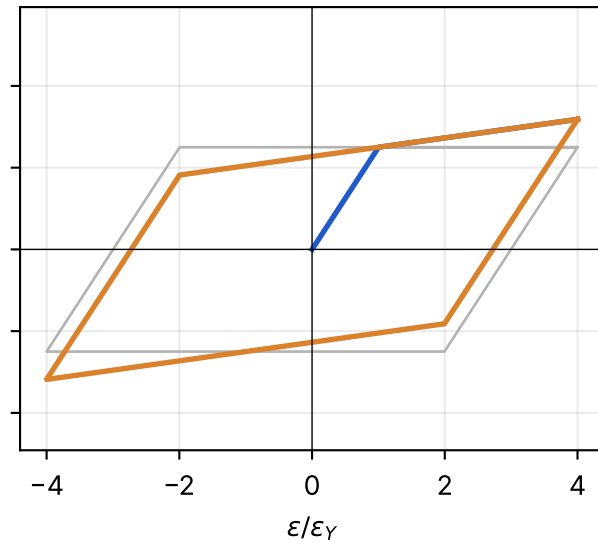
kinematic ( K=0 GPa, H=20 GPa)
