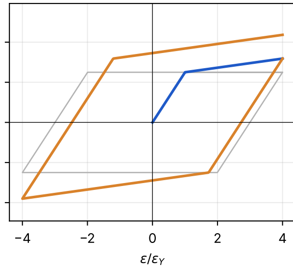
combined ( K=10 GPa, H=10 GPa)
