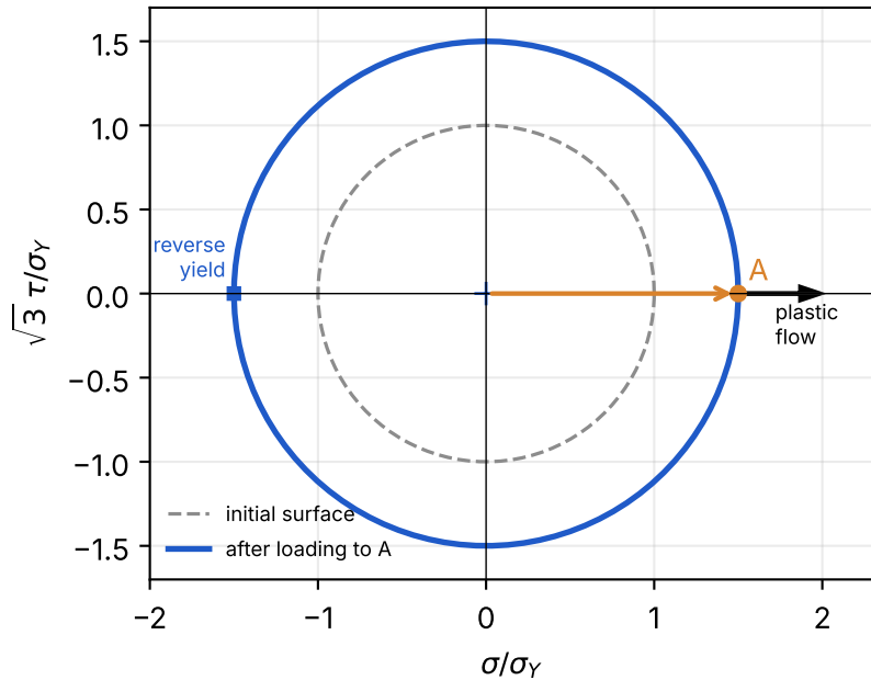
isotropic hardening
