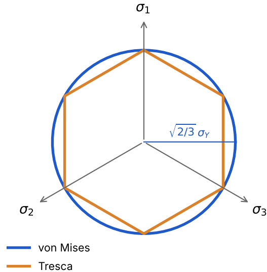
(b) deviatoric ( \pi ) plane
