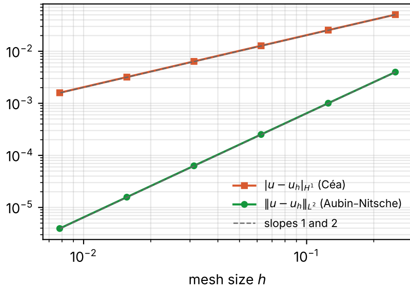
(b) finite elements, consistent load
