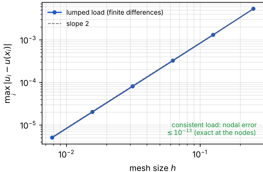
(a) nodal error
