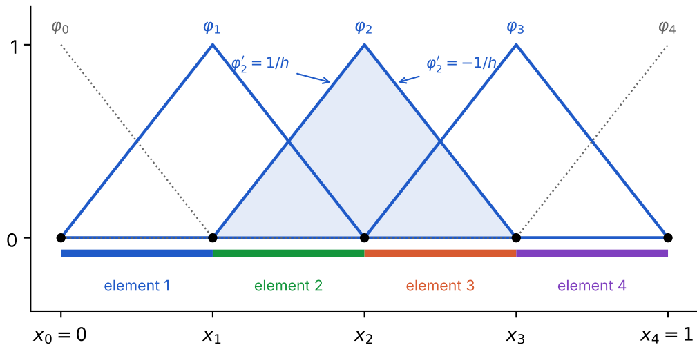
(a) hat functions; the end ones (dotted) are removed by u(0) = u(1) = 0
