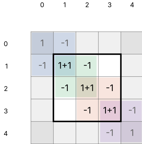
h \mathbf{K} : the framed block is tridiag(-1, 2, -1)
