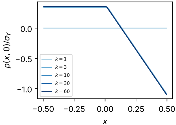
(b) residual stress through the wall
