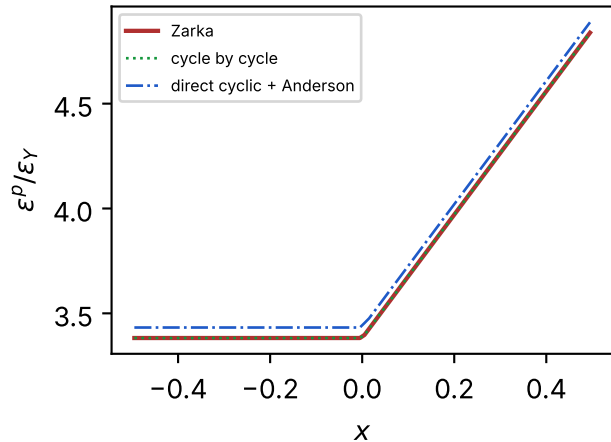
(b) shakedown plastic strain
