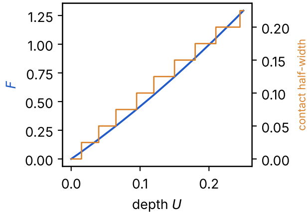
(b) force--depth curve
