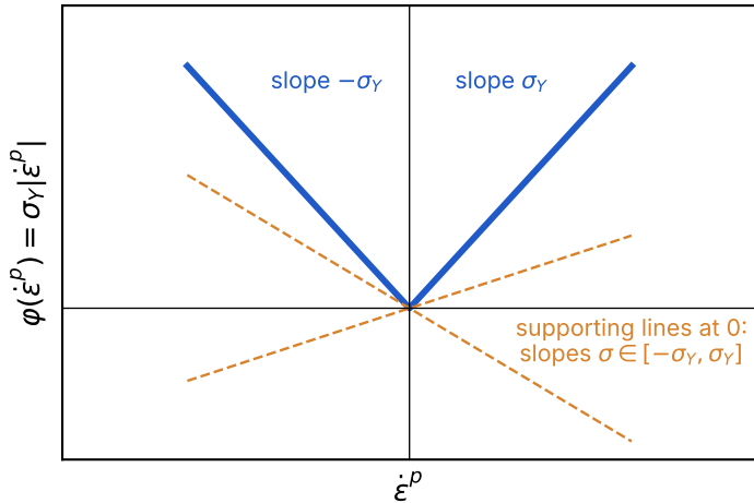
(a) dissipation potential \varphi
