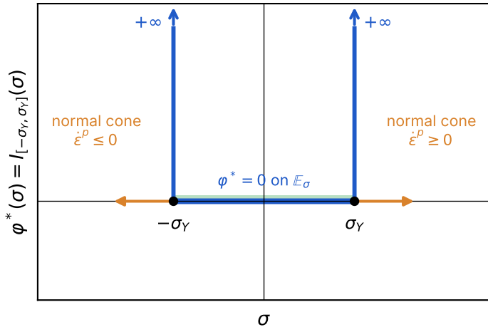
(b) its conjugate \varphi^* : indicator of \mathbb{E}_\sigma
