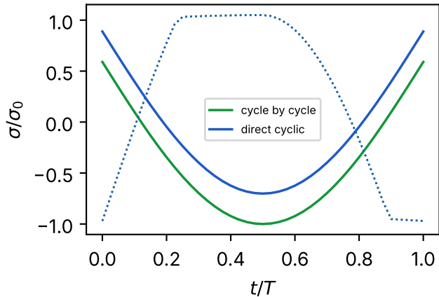
(a) stress cycles at x = -0.27 (dotted: outer skin)
