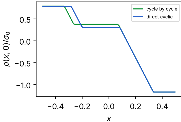
(b) residual stress at t = 0
