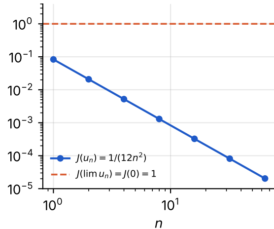
(c) J(u_n) \rightarrow 0 = \inf J , never attained
