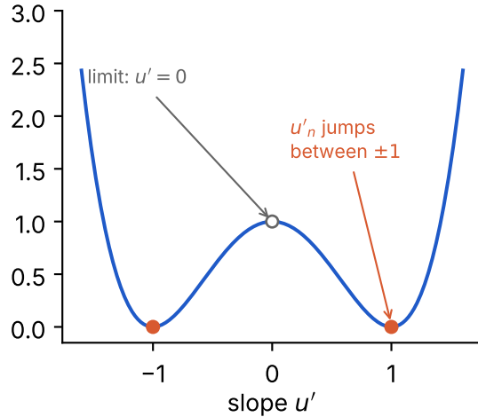
(b) non-convex density ((u')^2 - 1)^2
