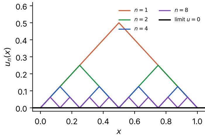
(a) sawtooth u_n , slopes \pm 1
