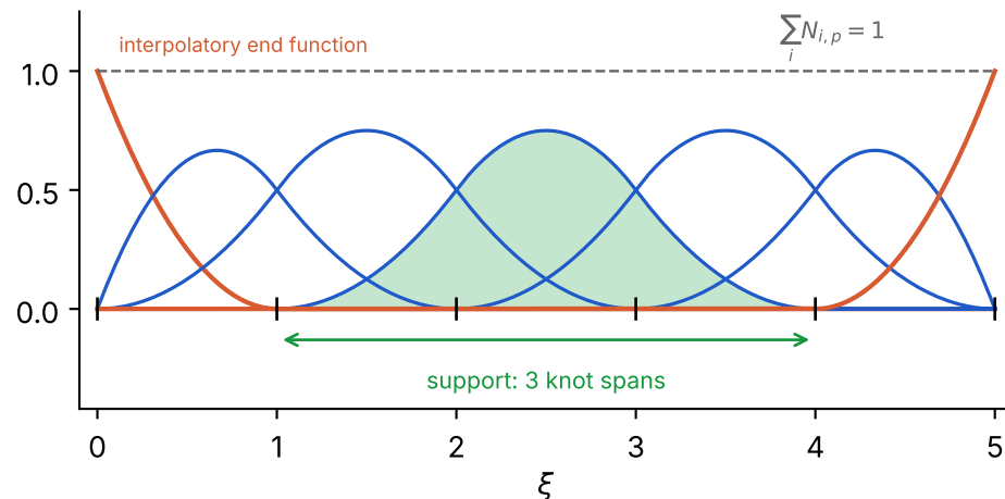
(b) p = 2 : quadratic B-splines, C^1
