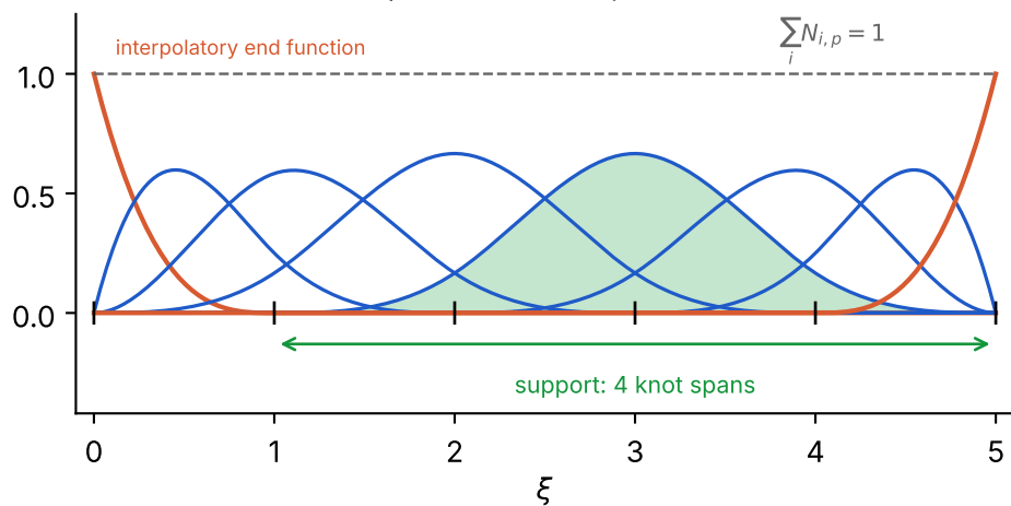
(c) p = 3 : cubic B-splines, C^2
